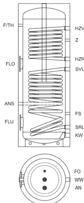
BRR 600
